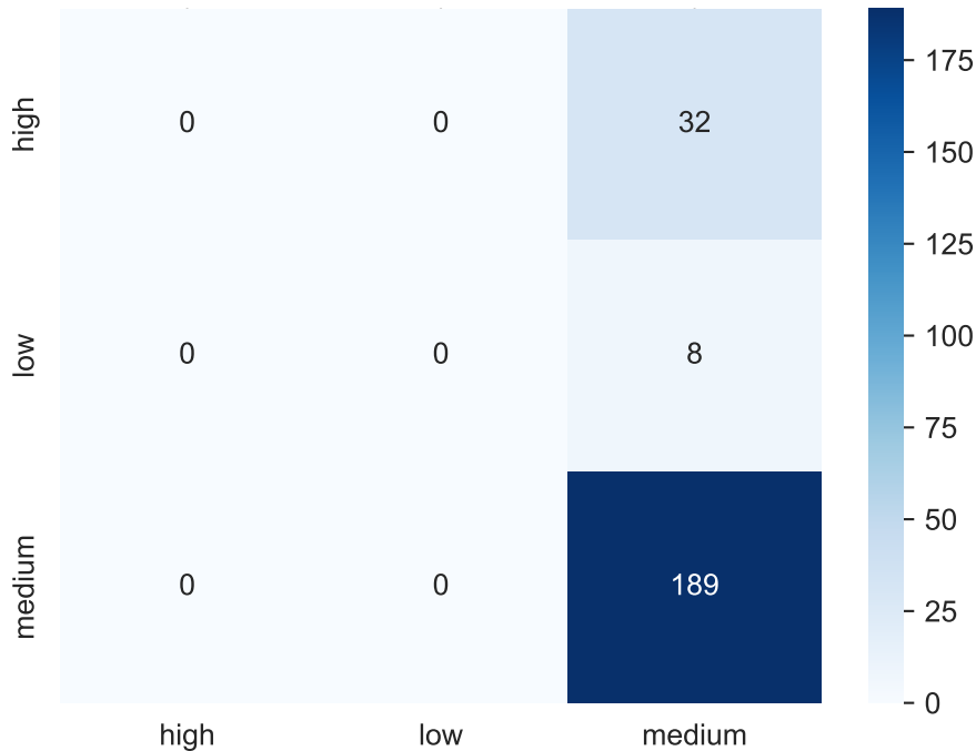
Confusion Matrix — SVC
